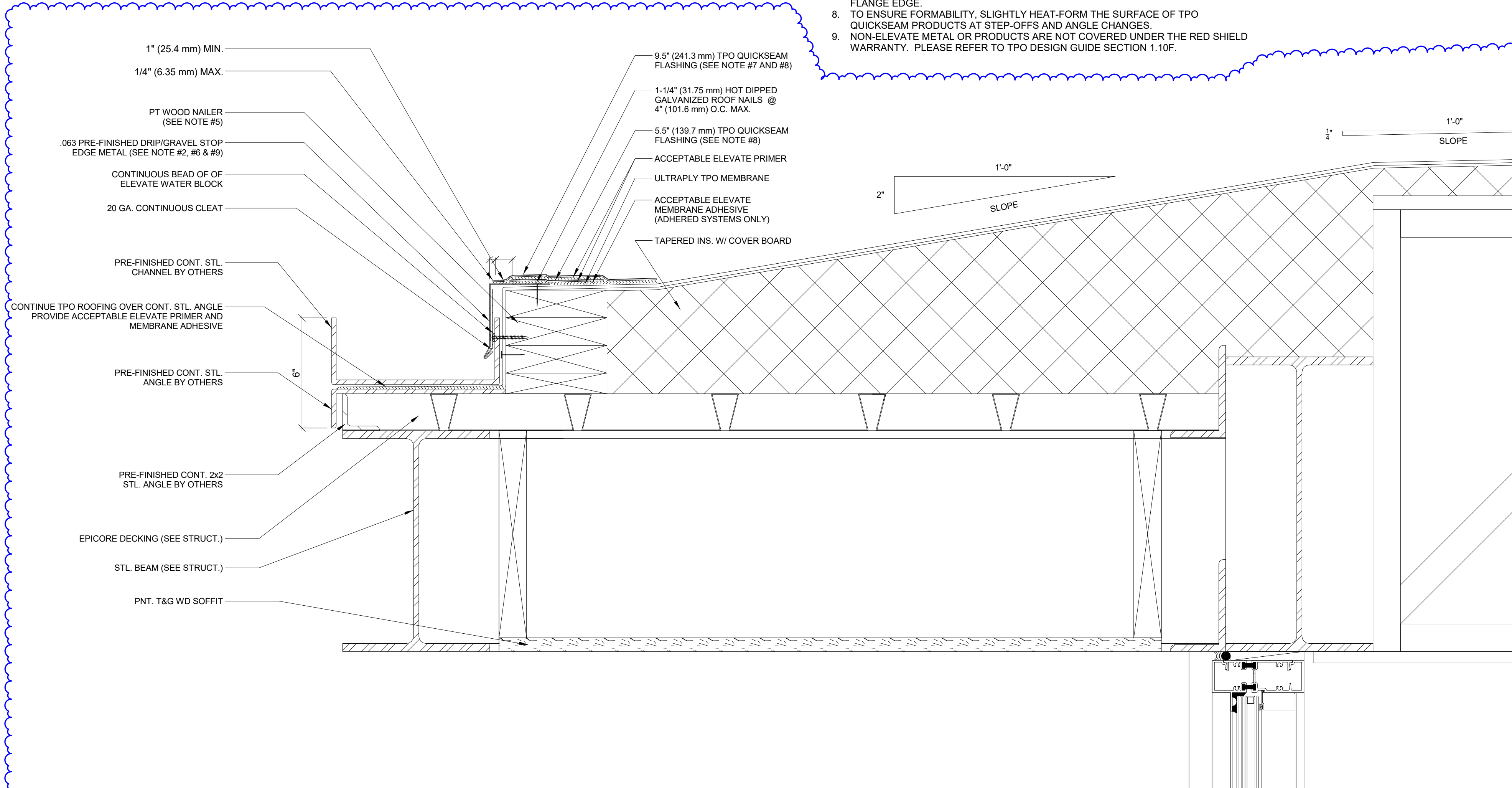
ROOF DETAIL - CURB / SKYLIGHT DTL 3" = 1'-0"
