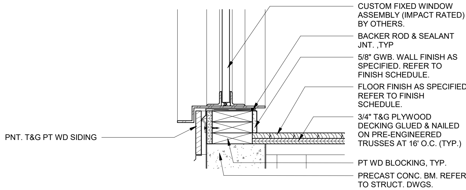
WINDOW - FIXED @ CONC BM - SILL DTL 1 1/2" = 1'-0"
