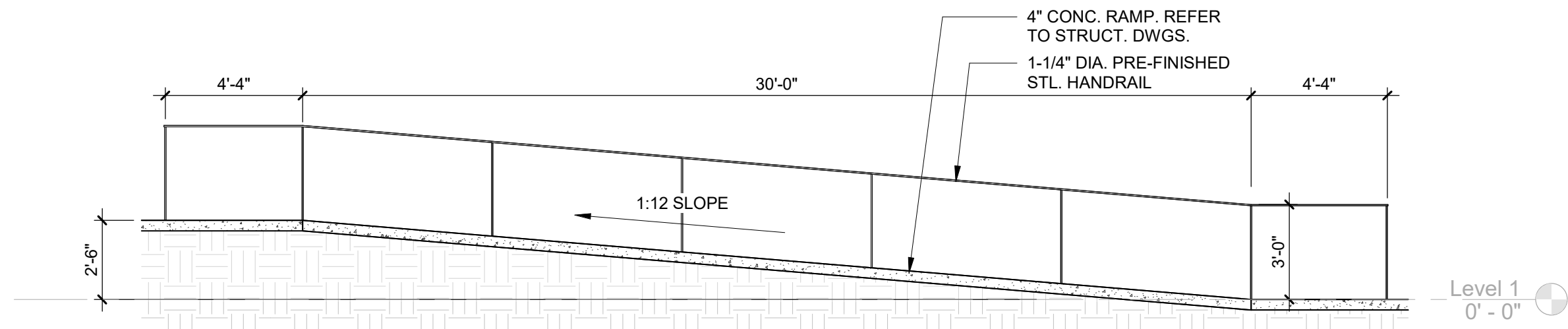
CIRCULATION SECTION - SITE RAMP 1/4" = 1'-0"
