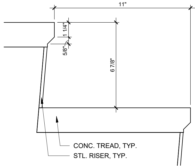
TYPICAL TREAD & RISER DETAIL 3" = 1'-0"
