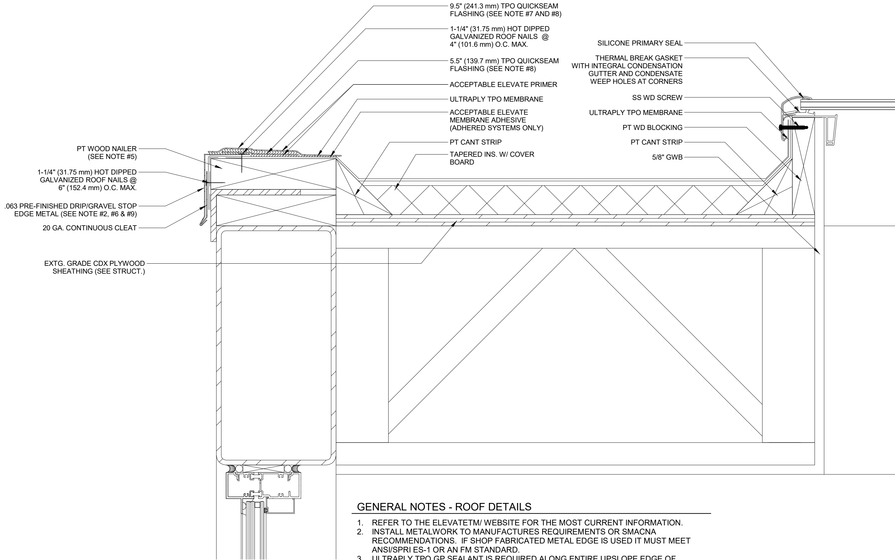
ROOF DETAIL - GARAGE - SKYLIGHT 3" = 1'-0"
