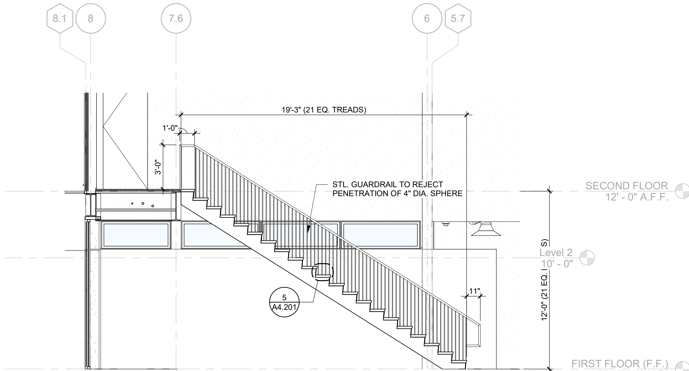
CIRCULATION SECTION - ATRIUM STAIR 1/4" = 1'-0"
