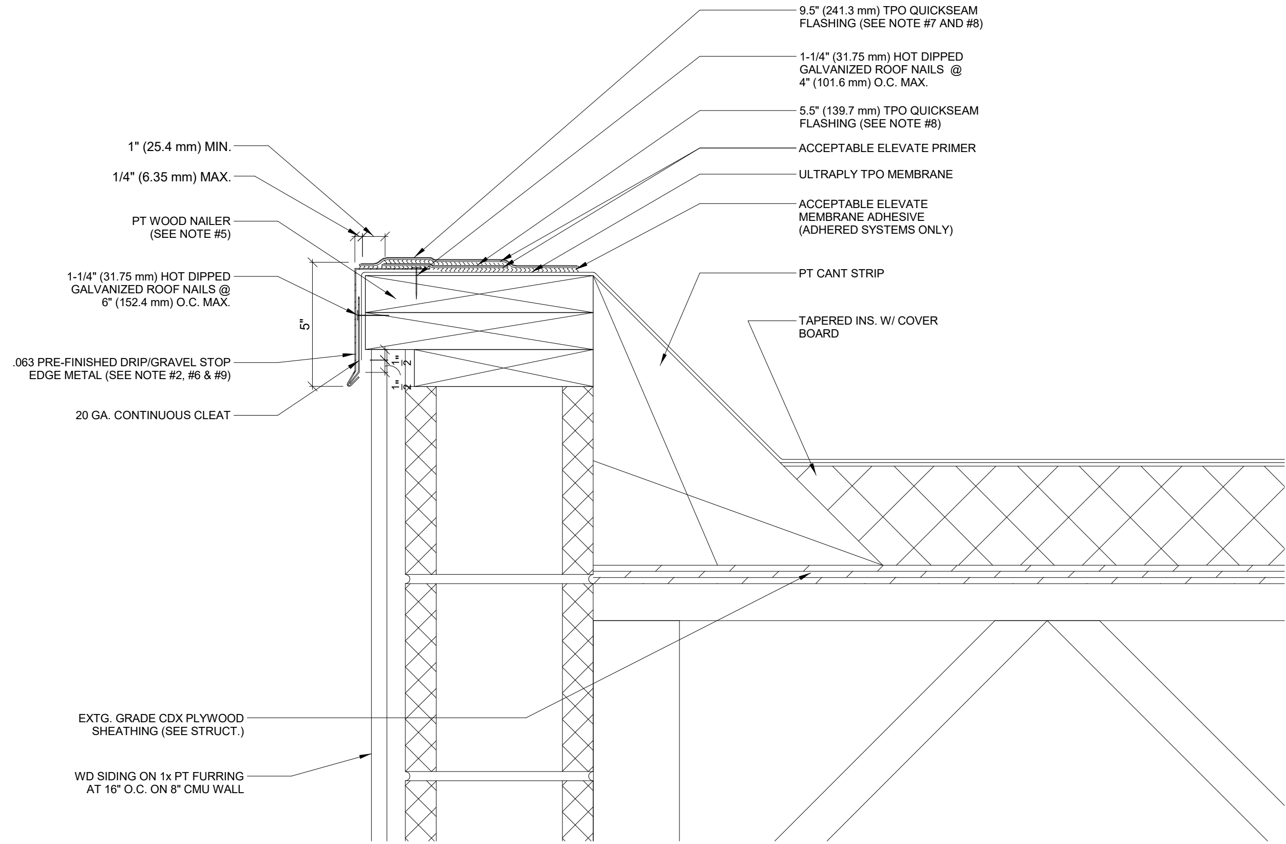
ROOF DETAIL - GARAGE - PARAPET 3" = 1'-0" 4
