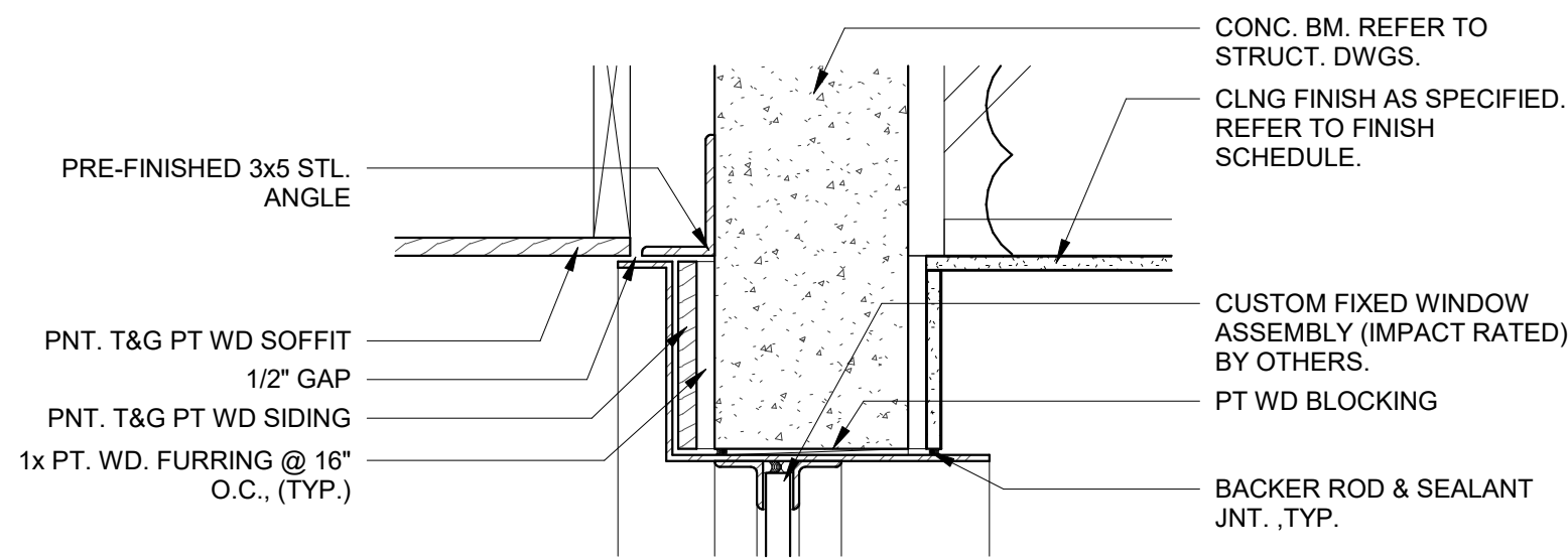
WINDOW - FIXED @ CONC BM - HEAD DTL 1 1/2" = 1'-0"
