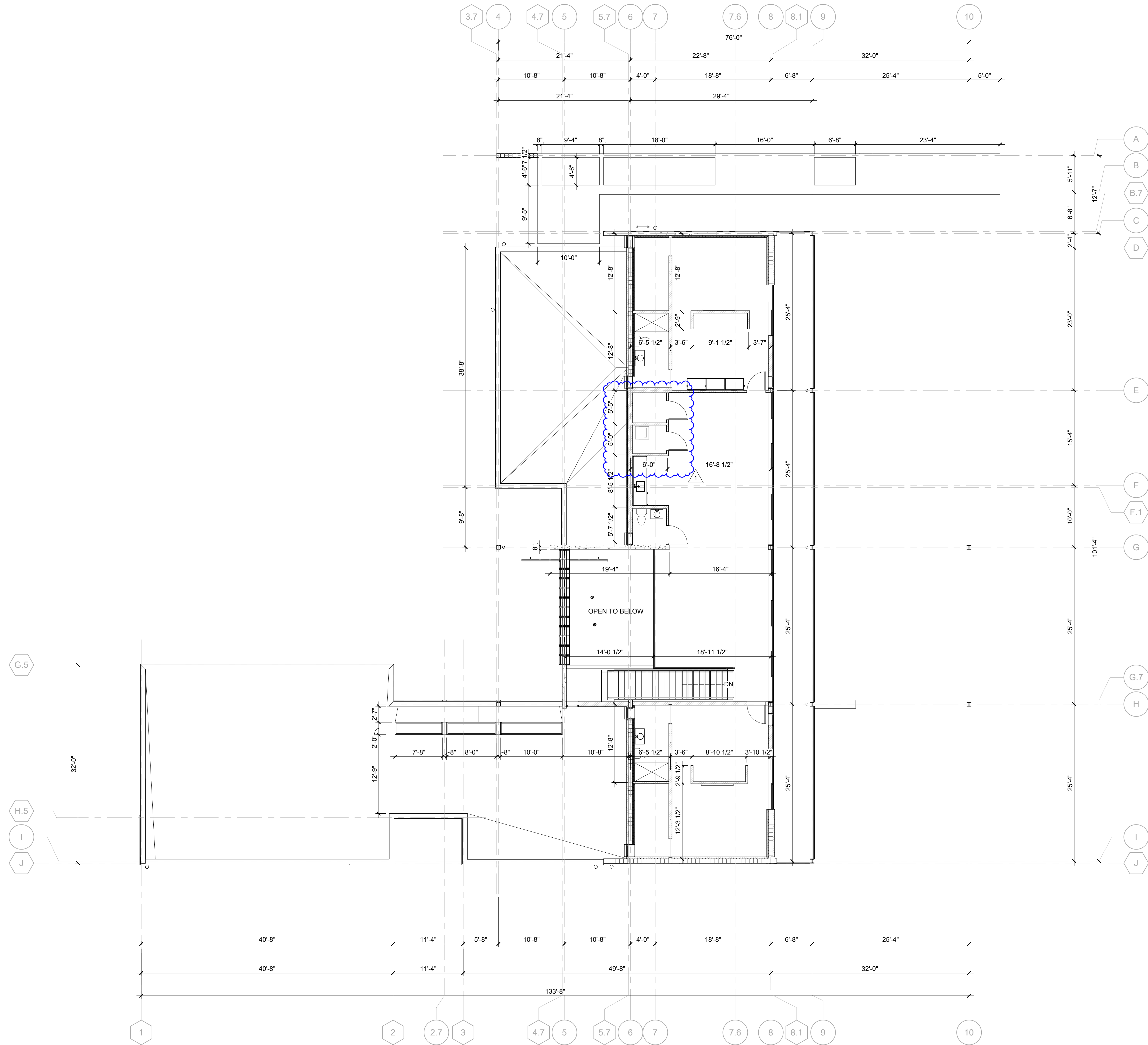
SECOND FLOOR DIMENSION PLAN
