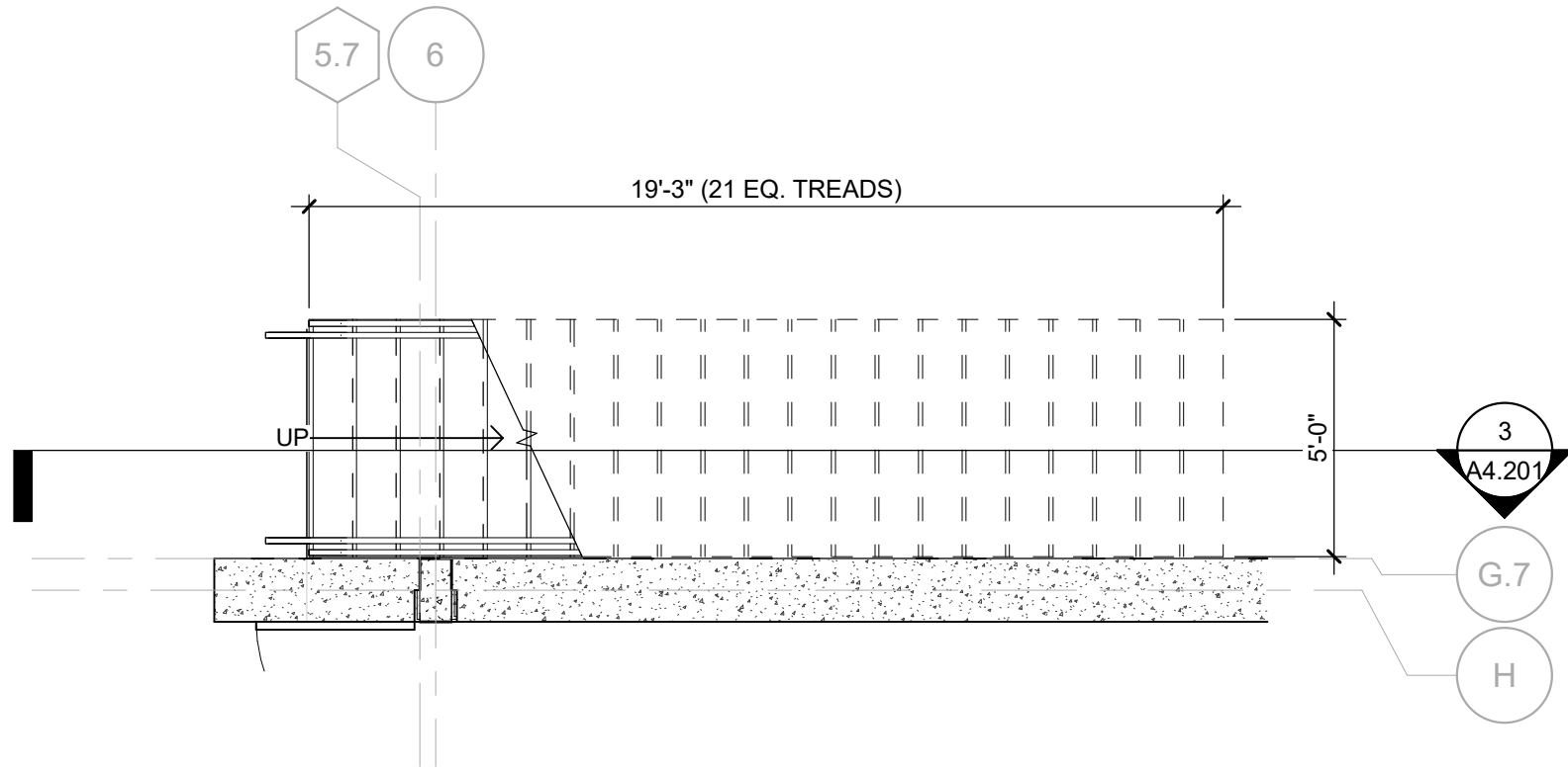
CIRCULATION PLAN - ATRIUM STAIR - FIRST FLOOR 1/4" = 1'-0"
