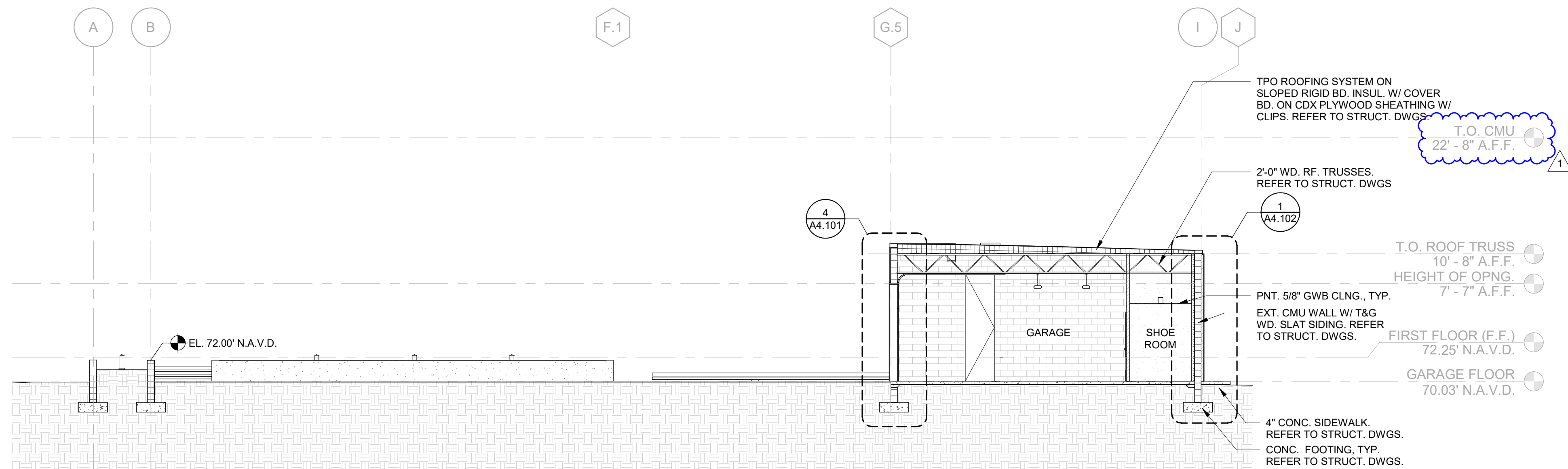
BUILDING SECTION E/W 1/8" = 1'-0"
