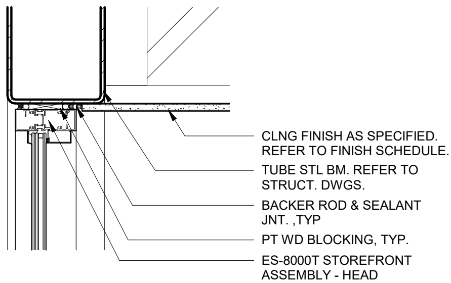
WINDOW - FIXED @ STL TUBE - HEAD DTL 1 1/2" = 1'-0"
