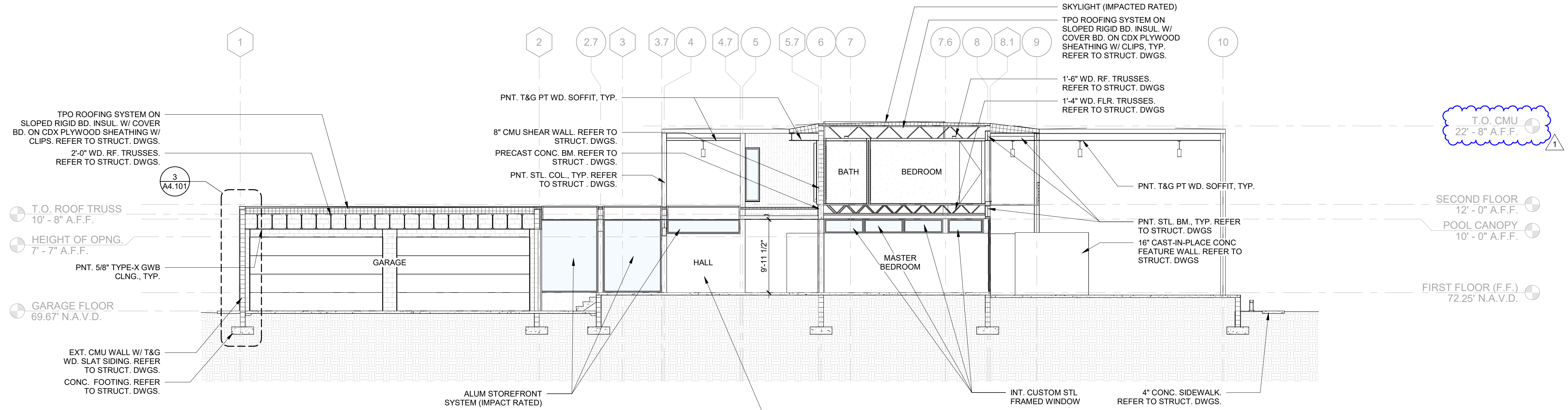
BUILDING SECTION E/W 1 1/8" = 1'-0"
