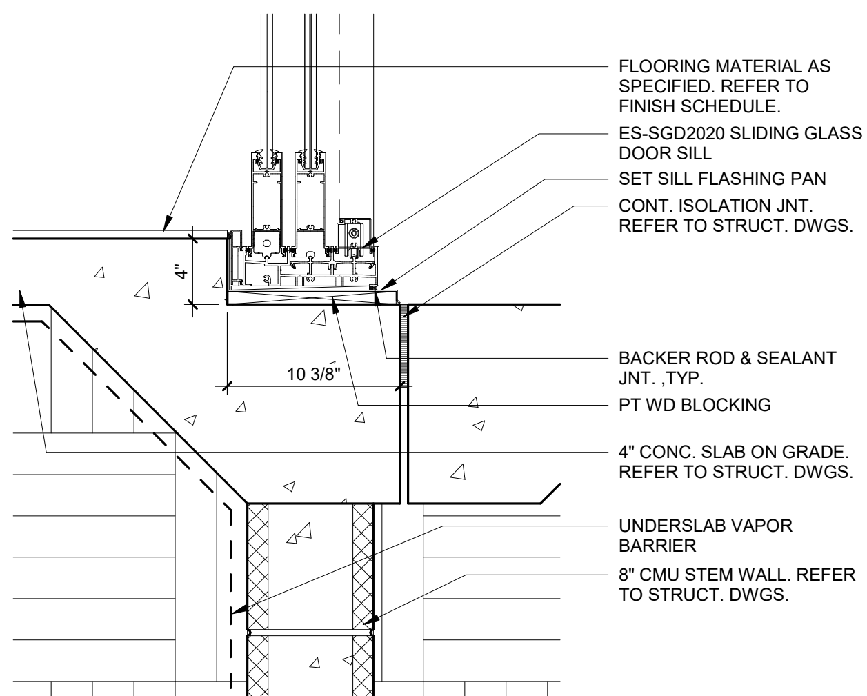
SLIDING DOOR @ L1 / EAST FACADE - SILL DTL 1 1/2" = 1'-0"
