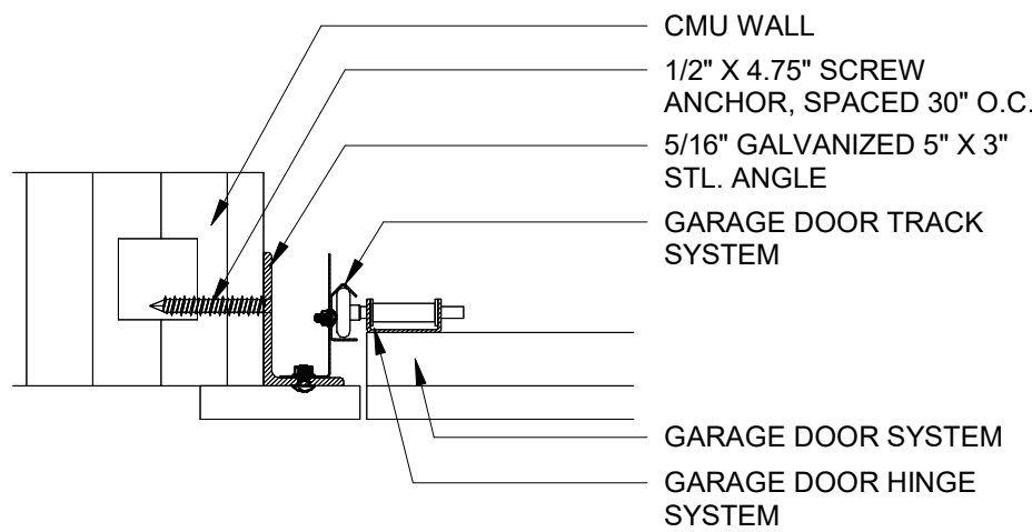
OVERHEAD DOOR - JAMB DTL 1 1/2" = 1'-0"
