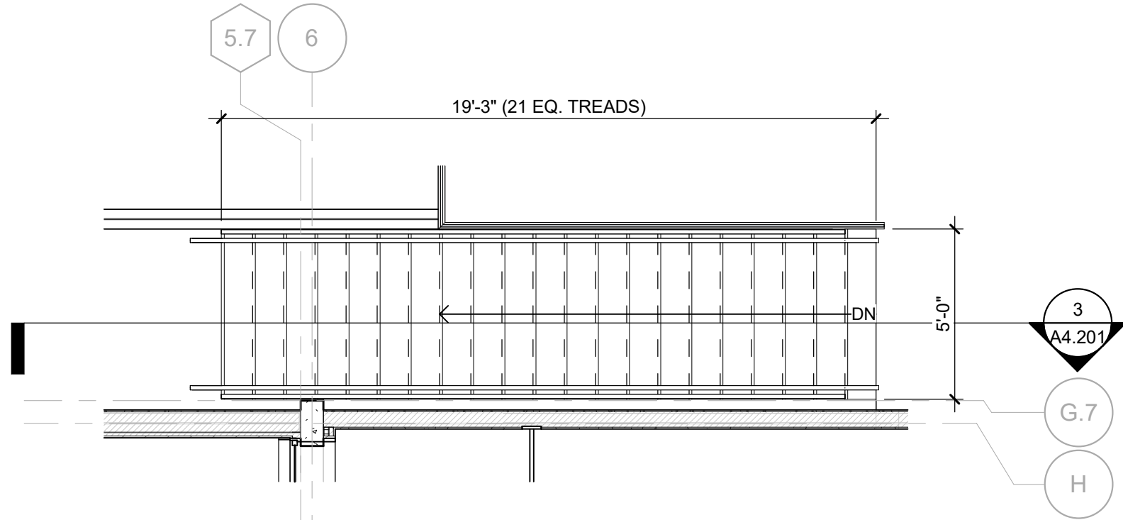
CIRCULATION PLAN - ATRIUM STAIR - SECOND FLOOR 1/4" = 1'-0"
