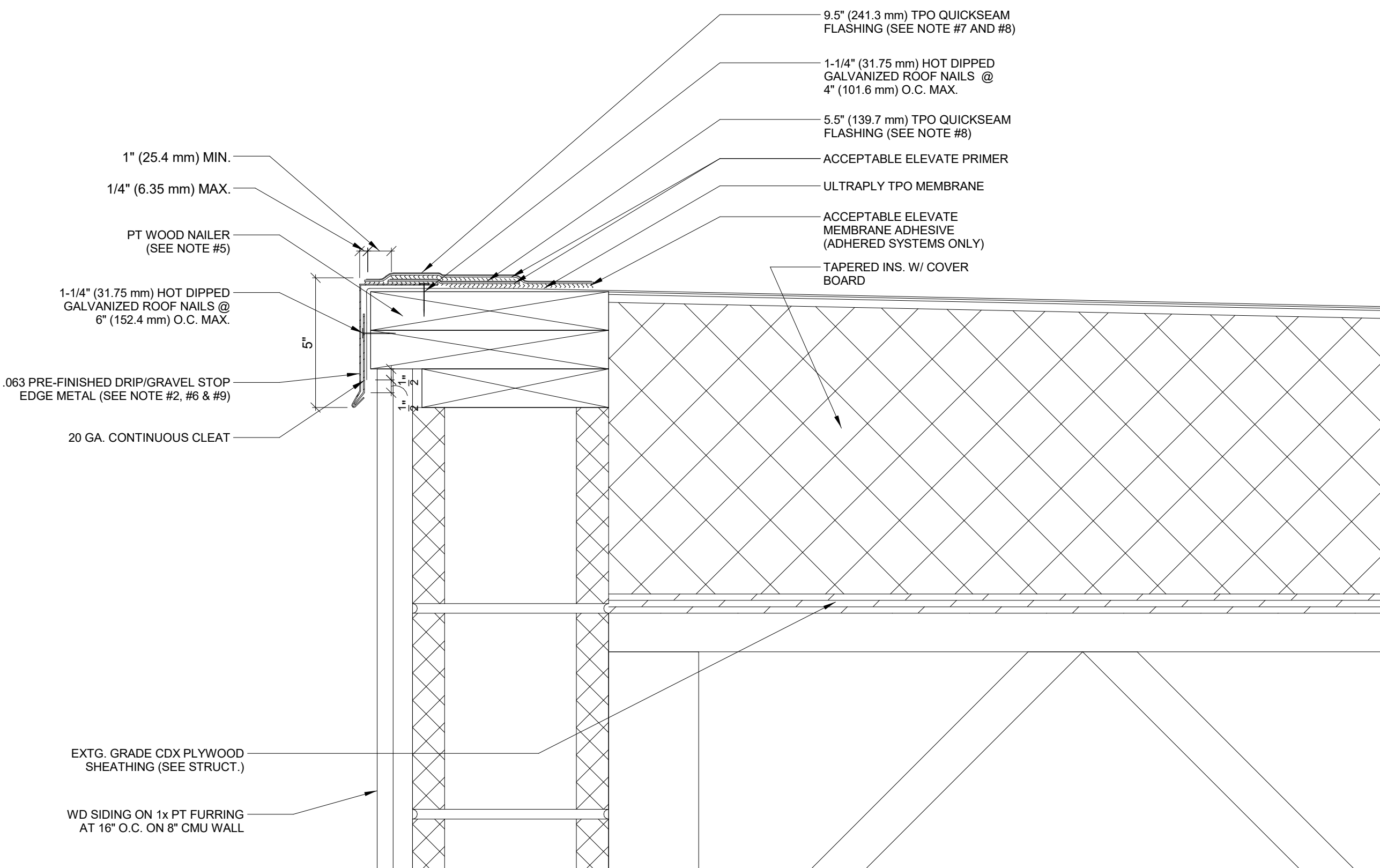
ROOF DETAIL - GARAGE - EDGE FLASHING 3" = 1'-0" 1
