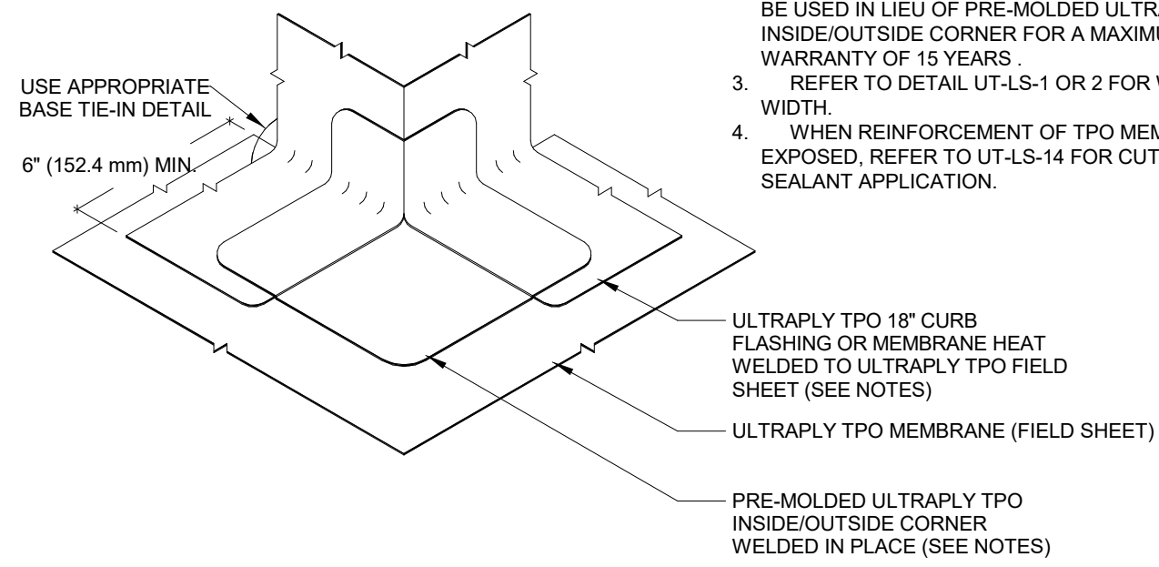
ROOF DETAIL - OUTSIDE CORNER DTL 3" = 1'-0"
