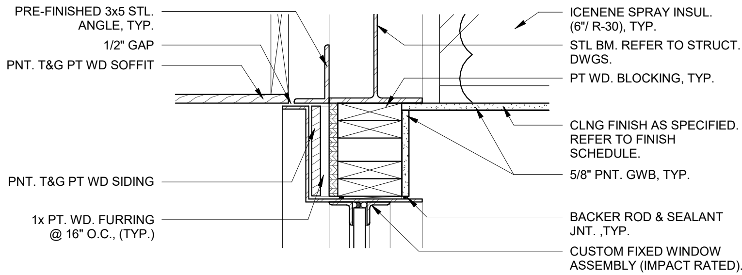
WINDOW - FIXED @ STL BM - HEAD DTL 1 1/2" = 1'-0"
