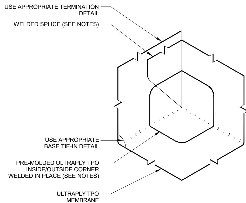
ROOF DETAIL - INSIDE CORNER DTL 3" = 1'-0"
