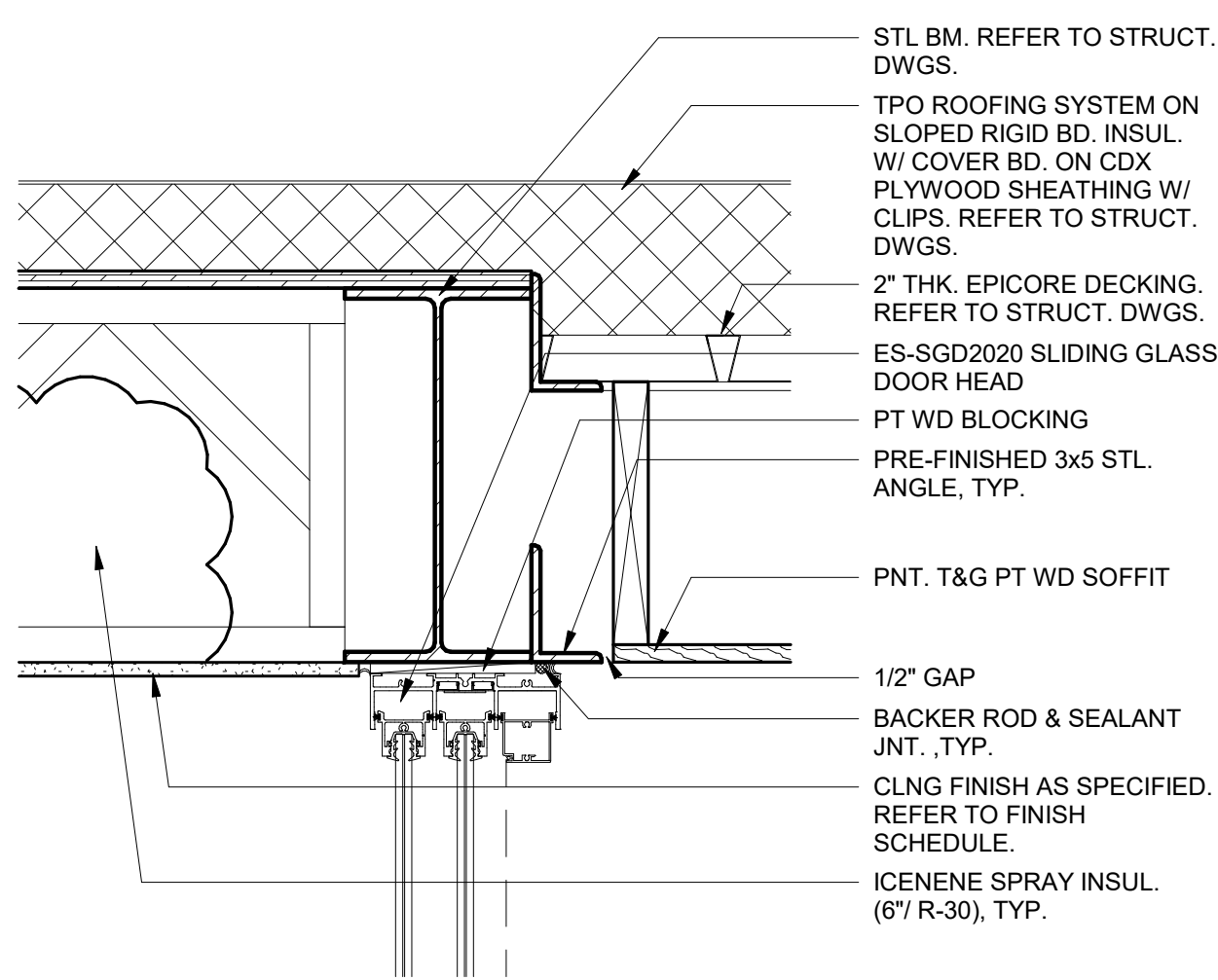
SLIDING DOOR @ L2 / EAST FACADE - HEAD DTL 1 1/2" = 1'-0"
