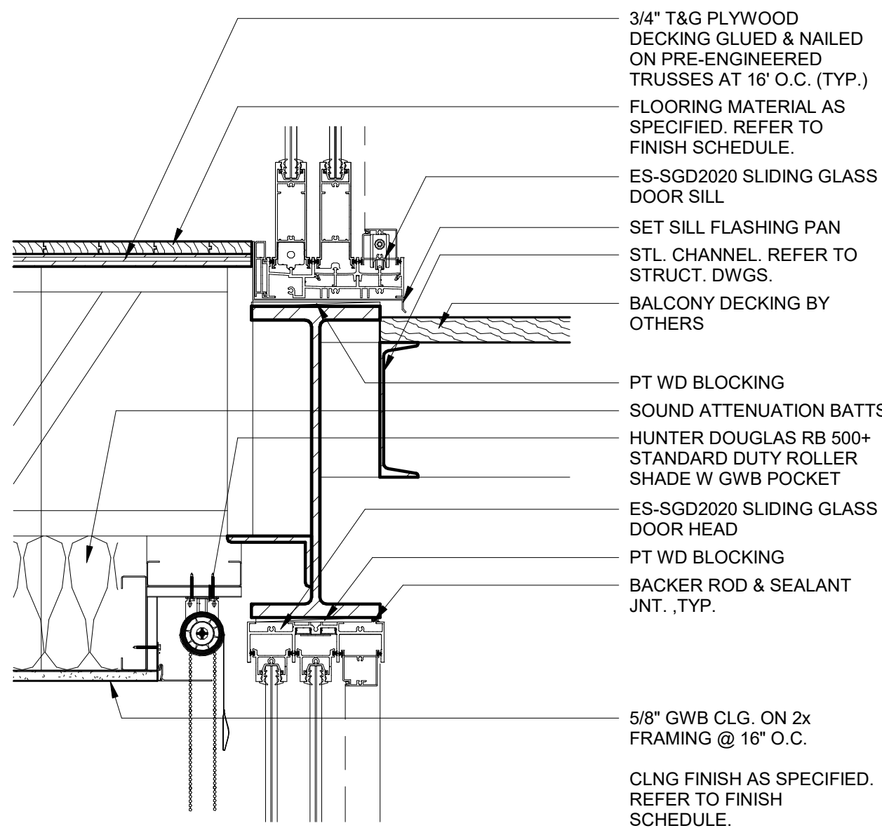
SLIDING DOOR @ L2 / EAST FACADE - HEAD DTL 1 1/2" = 1'-0"
