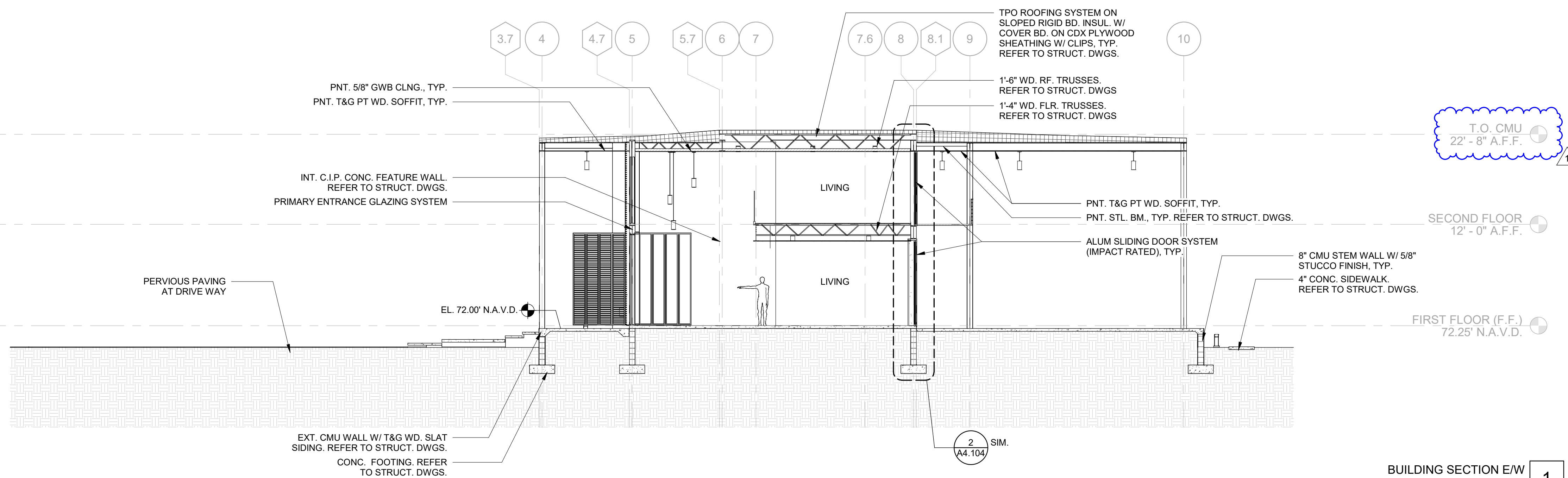
BUILDING SECTION E/W 1/8" = 1'-0"
