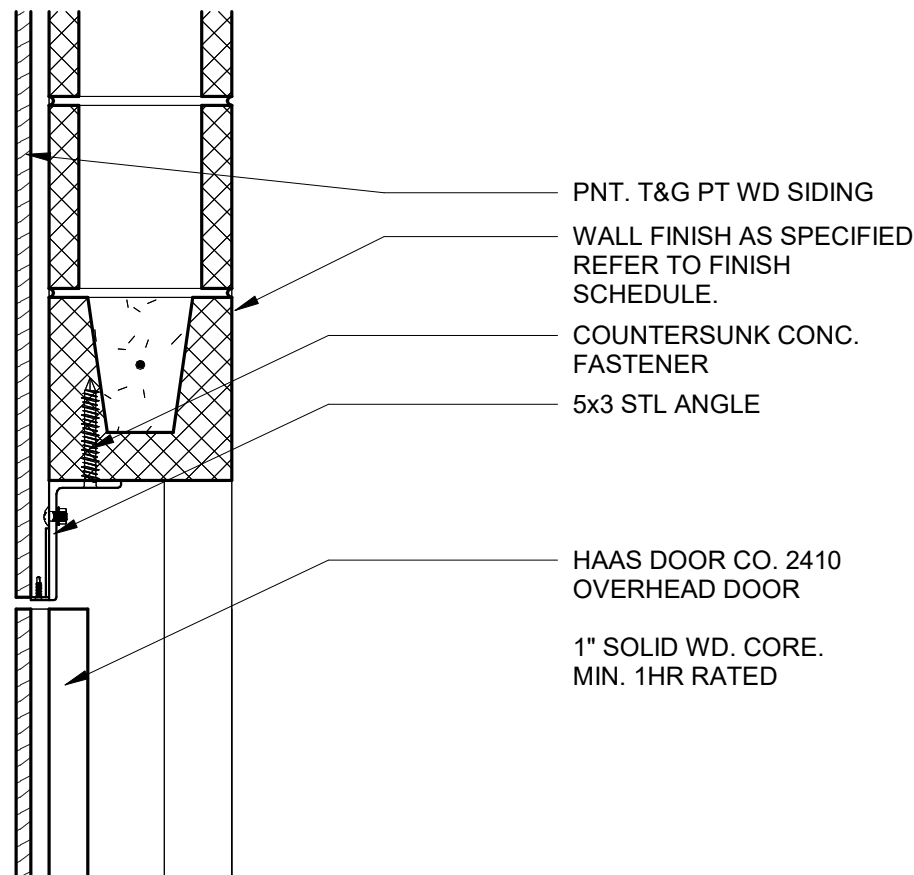
OVERHEAD DOOR - HEAD DTL 1 1/2" = 1'-0"
