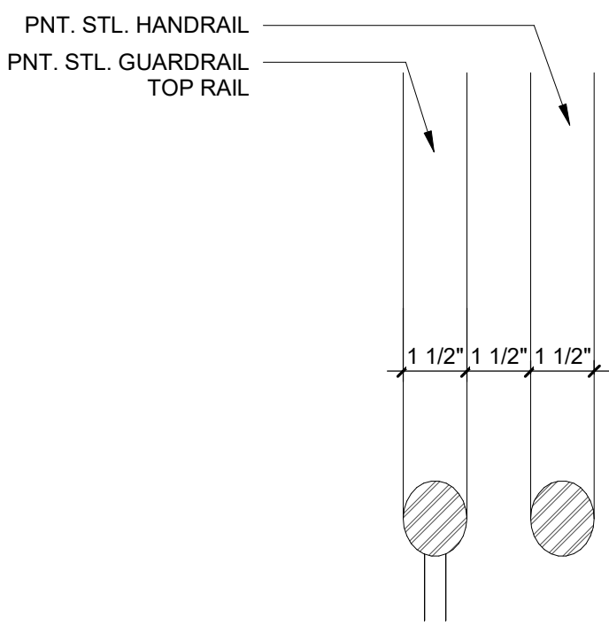
TYPICAL HANDRAIL CLEARANCE DETAIL 3" = 1'-0"
