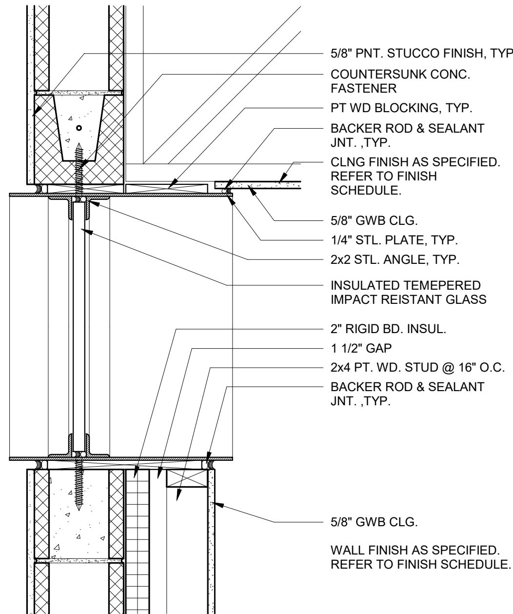
WINDOW - CUSTOM - HEAD / SILL DTL 1 1/2" = 1'-0"
